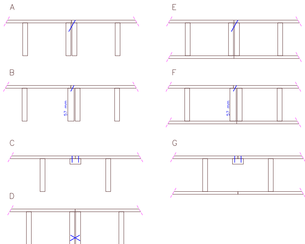
Figure 1-3: Principal drawing of connections between Kerto-Ripa Elements Guillet (KREG).
