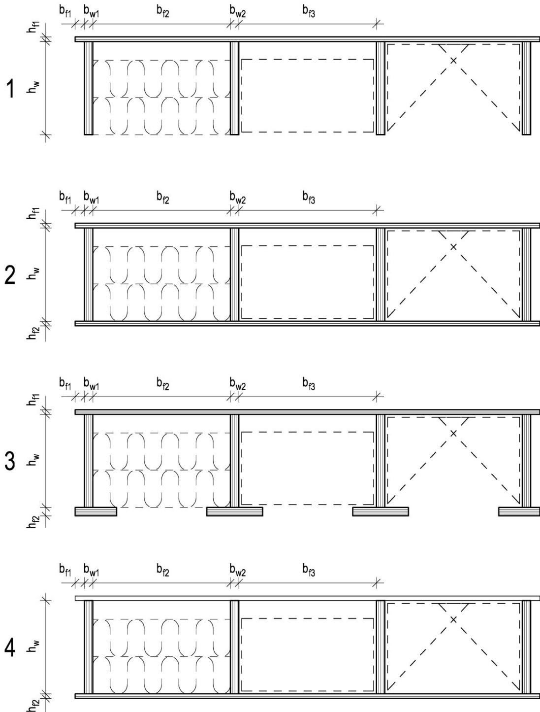
Figure 1-1: Cross sections of Kerto-Ripa Elements Guillet (KREG): 1 Ribbed slab, 2 Box slab, 3 Open box slab with Kerto-S or Kerto-Q bottom flanges (depending on the design), may contain optional fire protective bottom courses, and 4 Box slab where top panel is not a part of the composite cross section. Cross bracing and insulation are optional.
